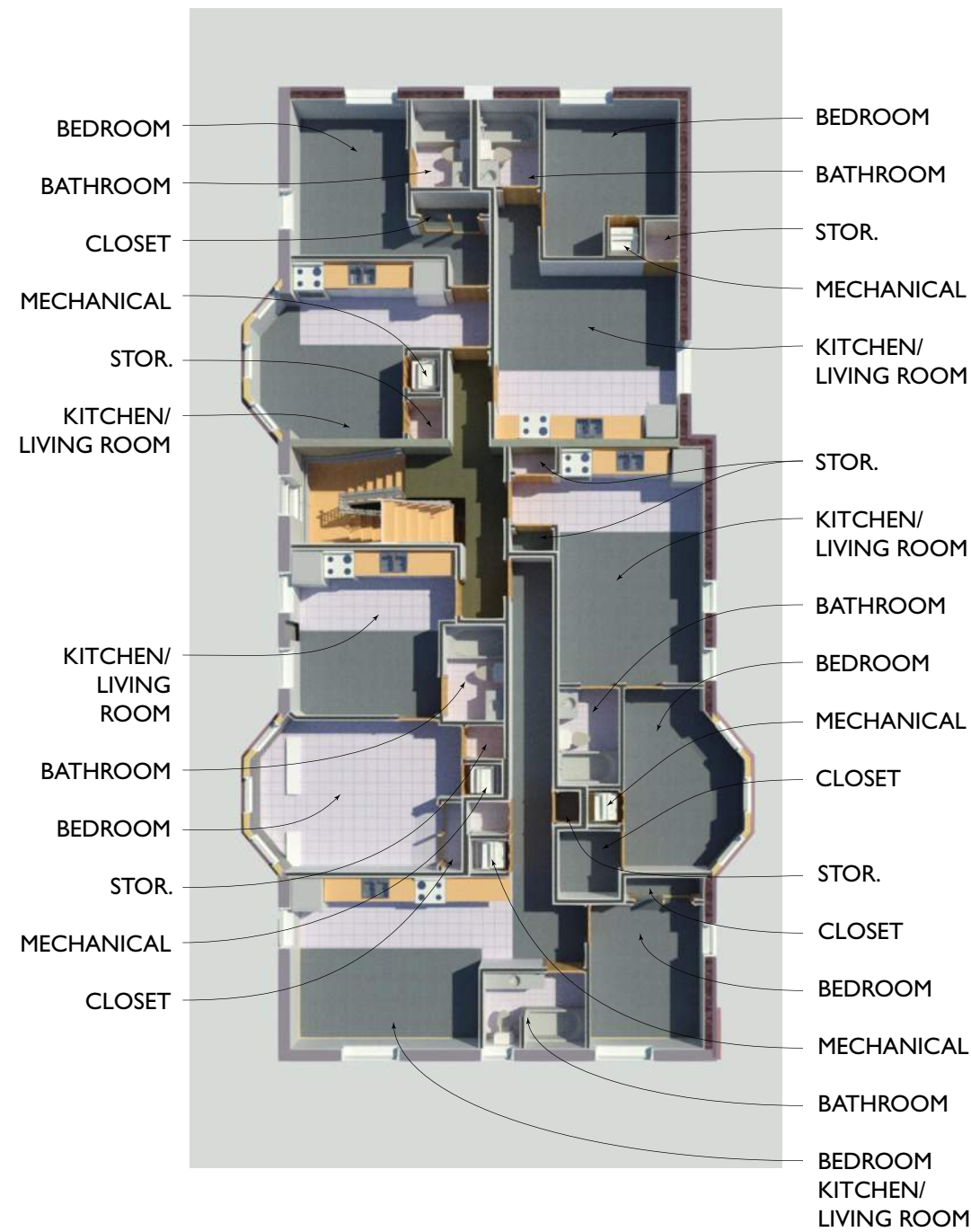
SECOND FLOOR (RESIDENTIAL)
